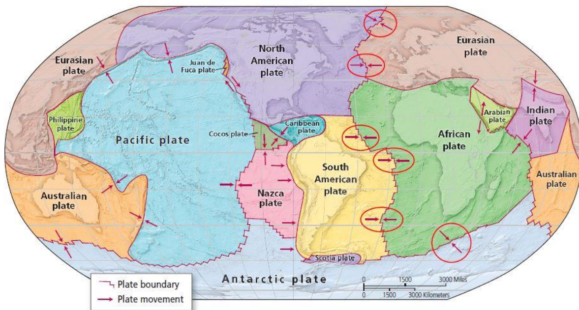
1.1 Plate boundaries
